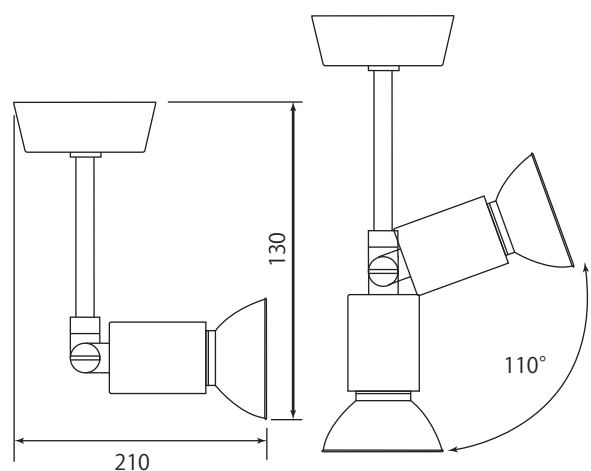
Profile sketch
